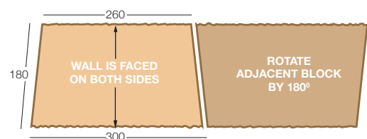
DOUBLE-SIDED WALL
